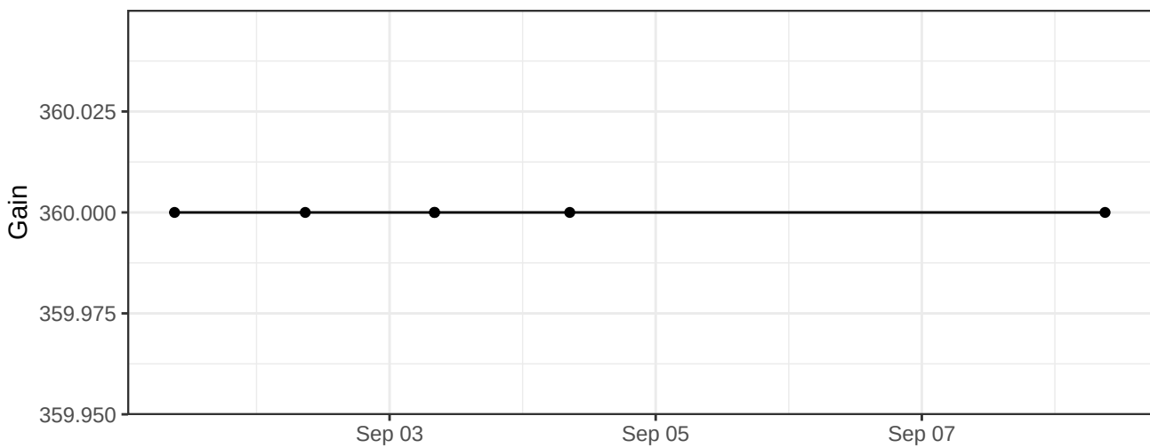
DAPI-A_Gain
